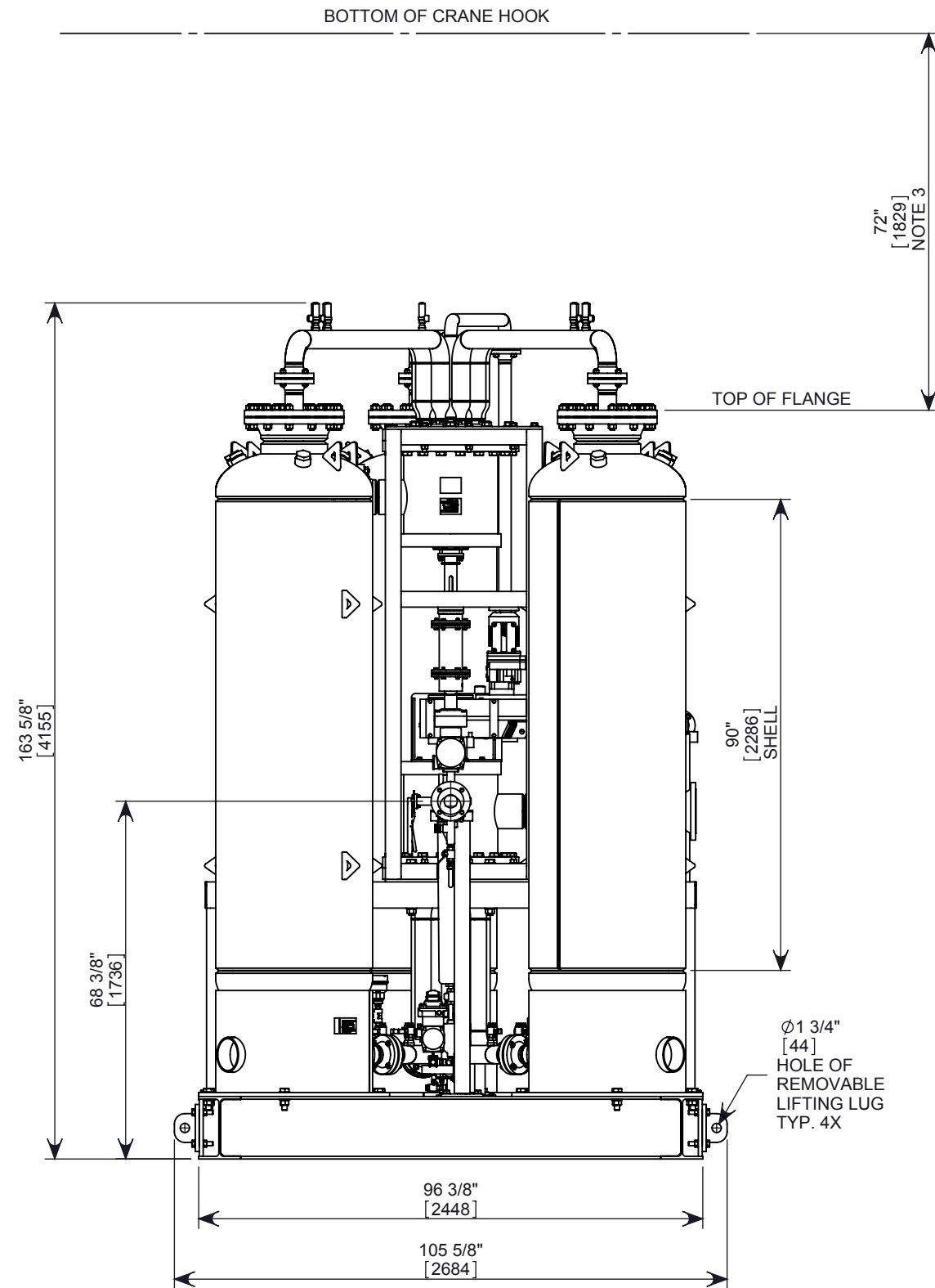
SIDE VIEW
