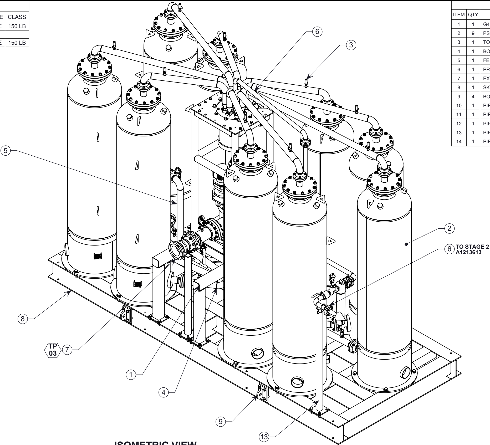
ISOMETRIC VIEW (FRONT)
