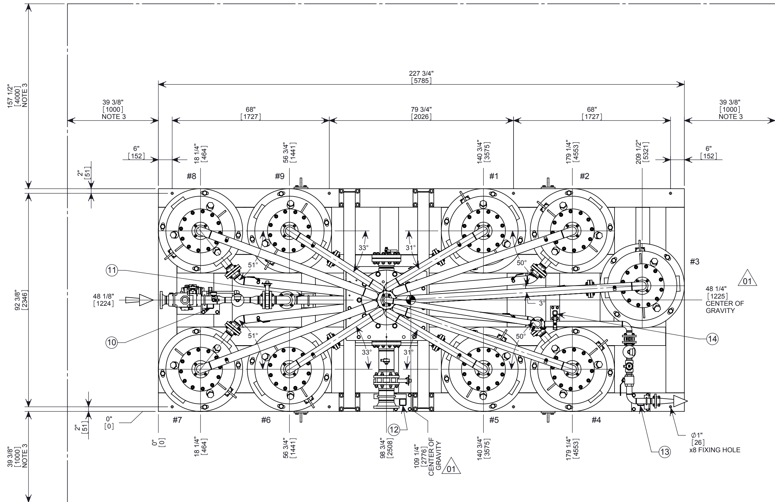
TOP VIEW
