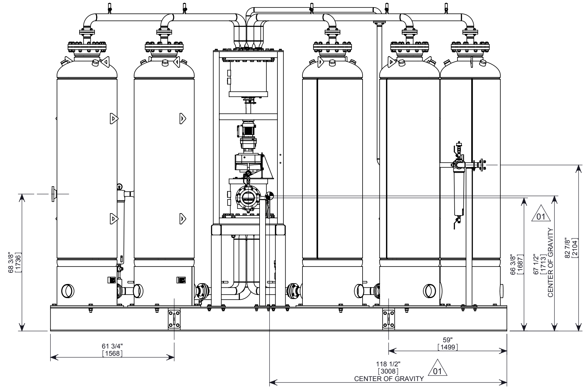
FRONT VIEW
